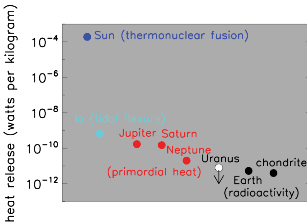
FIGURE 7.4 The intrinsic specific luminosities of some solar system objects are arrayed horizontally by predominant regimes of internal heat production at the present epoch. The Sun (blue) derives quasi-steady heating through thermonuclear fusion, while heating from tidal flexure is important in Io (light blue) and possibly in some exoplanets. Jupiter, Saturn, and Neptune (red) predominantly release primordial accretional heat. In Earth and other rocky objects of roughly chondritic composition (black), radioactive decay is important for heat production. SOURCE: Courtesy of William Hubbard.
