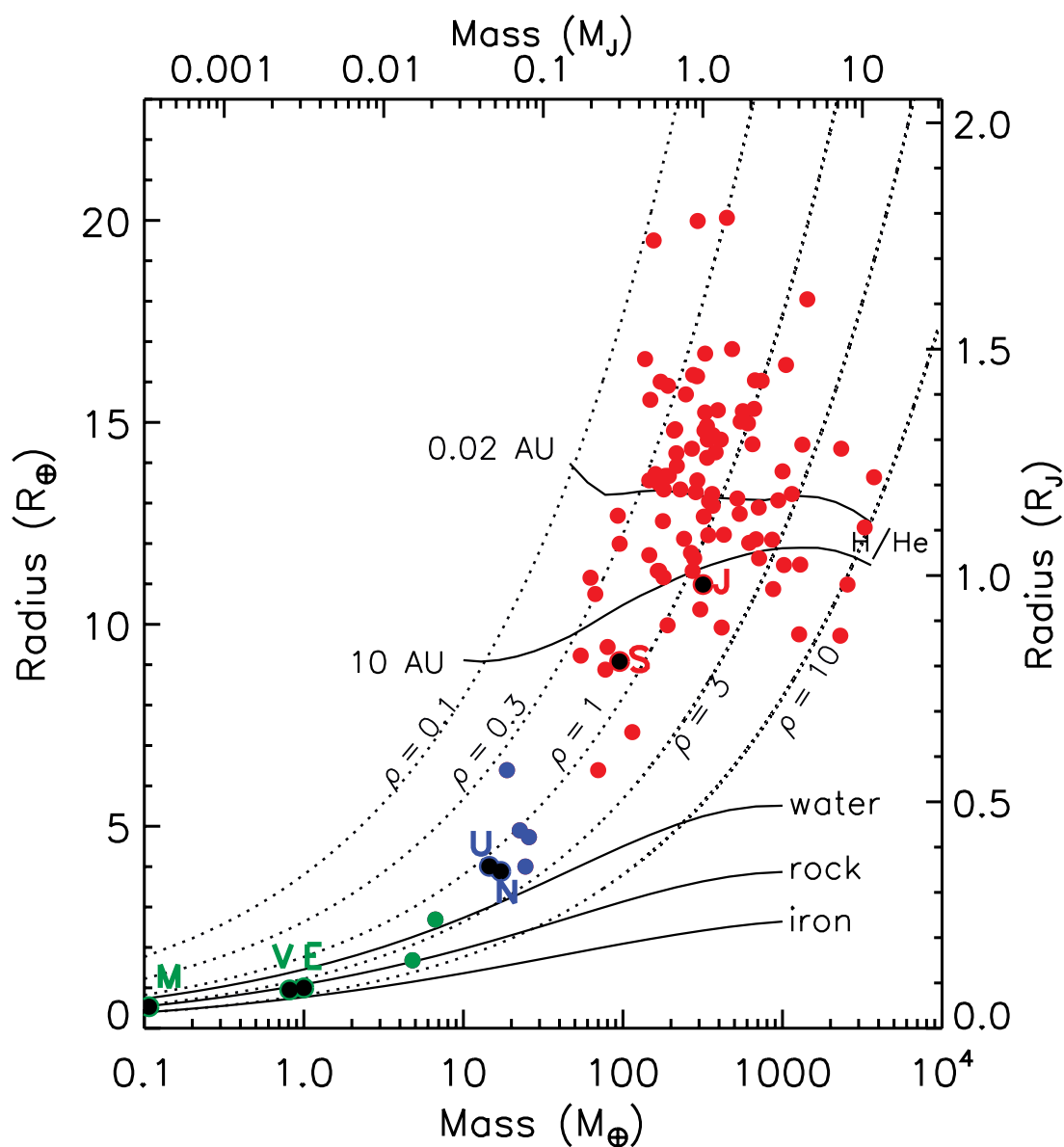
FIGURE 7.9 Planets now fill a continuum of sizes and distances from their host stars. In this mass-radius (MR) diagram, seven solar system planets (black circles with letters; M = Mars) are compared with transiting exoplanets: gas-giant exoplanets (red circles); ice-giant exoplanets (blue circles), and super-Earths (green circles). The three lower lines are theoretical MR relations for super-Earths lacking a hydrogen-helium envelope, but with three differing solid compositions (water-, silicate-, and iron-dominated). The lines denoted “H/He” in the cluster of giants mark the radius expected for coreless giant planets with an assumed age of 4.5 billion years at the indicated distance from their stars. Many objects, termed inflated giants , lie much higher than those lines, indicating that we do not yet understand giant-planet evolution under severe stellar insolation. The solar system’s gas giants Jupiter and Saturn have been studied in some detail; its ice giants Uranus and Neptune are less well understood. SOURCE: Courtesy of Jonathan Fortney.
