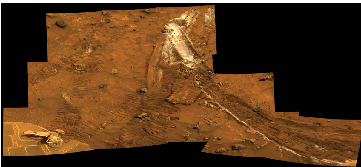
FIGURES 6.5 Top : Examples of the record of martian mineralogic diversity accessible from a surface rover mission. Bottom : Quartz-rich subsurface material exposed in the rover's tracks. These images were taken by Spirit on the south side of Husband Hill. Each rover track is 10 cm wide. SOURCE: NASA/JPL.
