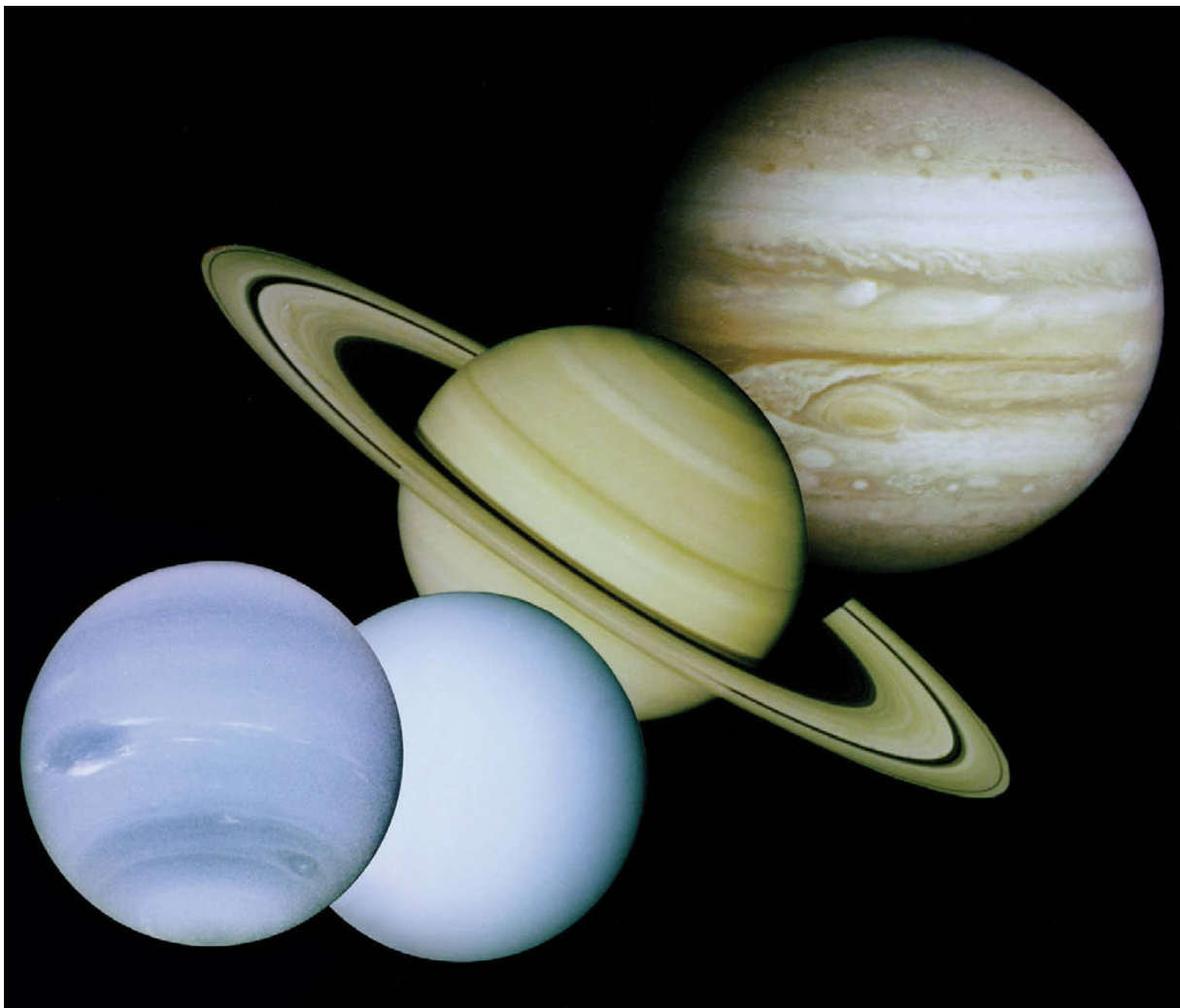
FIGURE 7.1 The giant planets—Neptune, Uranus, Saturn, and Jupiter—exhibit a diversity of properties and processes relevant to planetary science both in our local neighborhood of the solar system and in planetary systems discovered around nearby stars. SOURCE: NASA; available at http://www.astrophys-assist.com/educate/robot/page11.htm .
