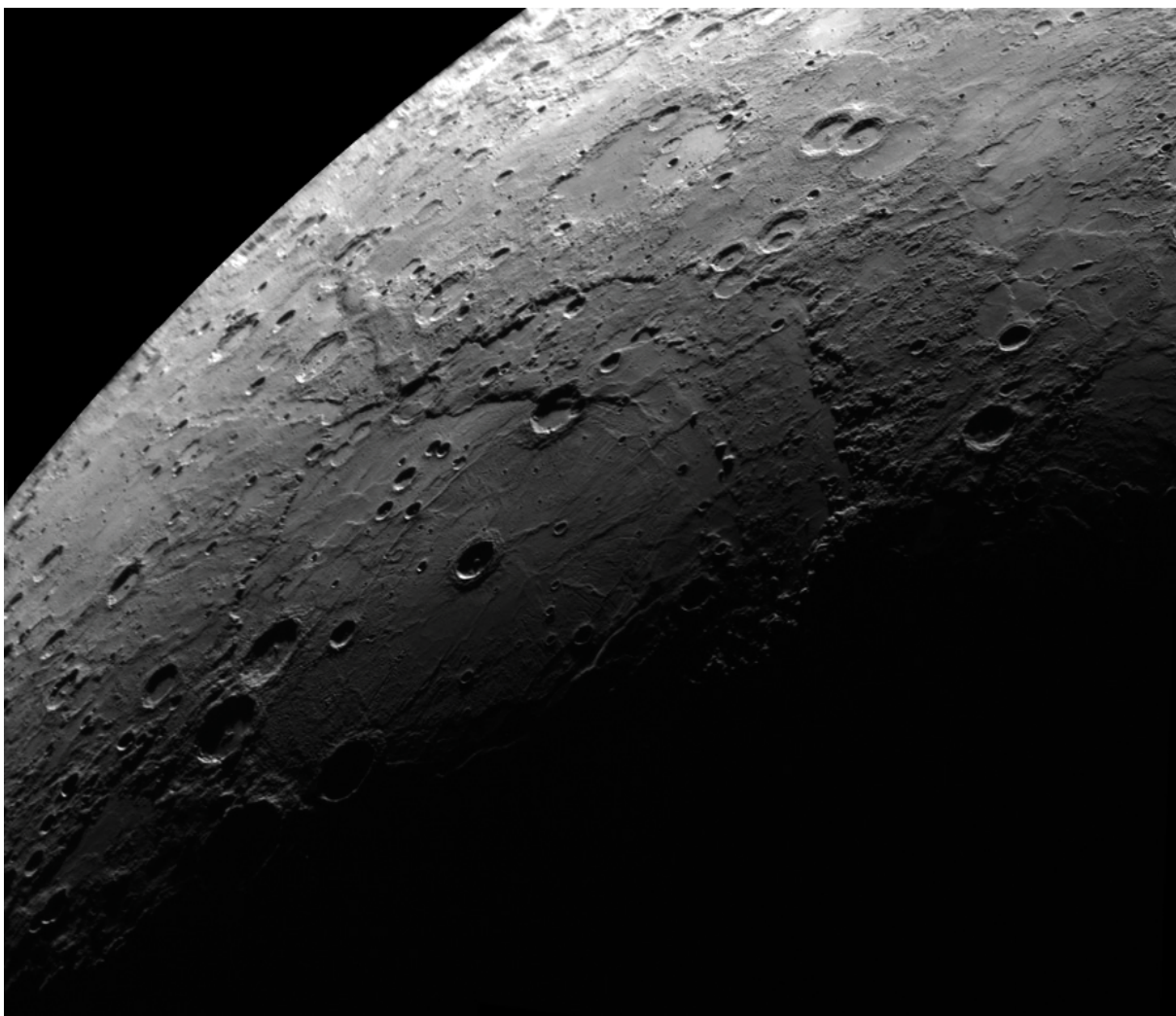
FIGURE 5.2 Rembrandt impact basin on Mercury photographed by MESSENGER. Rembrandt spans more than 700 km and at 4 billion years old is possibly the youngest large impact basin on the planet. Geologic analysis indicates that the basin experienced multiple stages of volcanic infilling and tectonic deformation. SOURCE: Courtesy of NASA/Johns Hopkins University Applied Physics Laboratory/Carnegie Institution of Washington, from the cover of Science , Vol. 324, No. 5927, May 1, 2009; reprinted with permission from AAAS.
