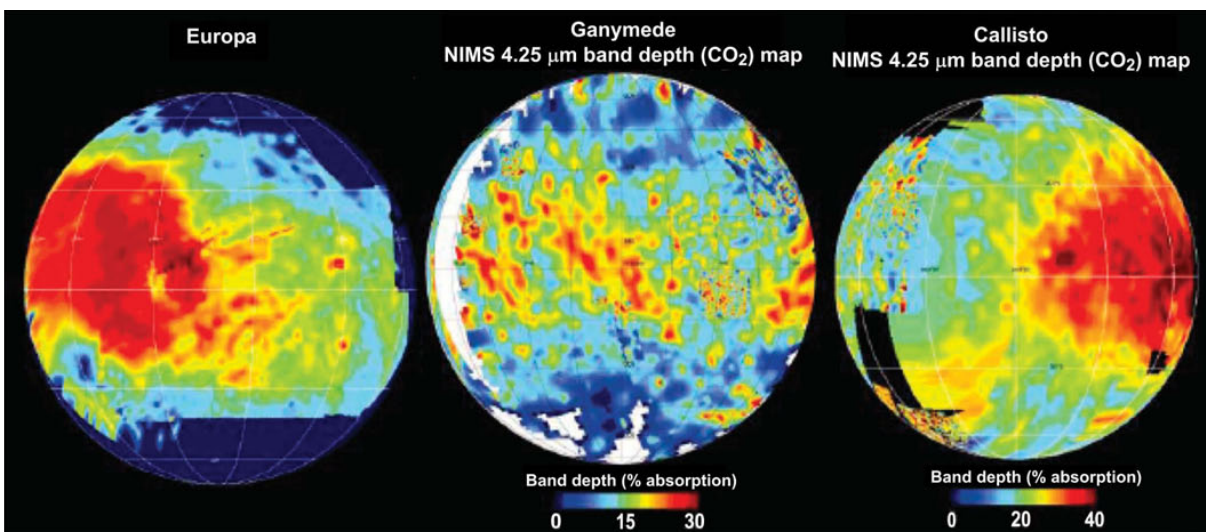
FIGURE 8.9 Near-infrared maps from the Galileo mission of non-water-ice surface materials on Europa ( left , sulfate hydrates), Ganymede ( middle , carbon dioxide), and Callisto ( right , carbon dioxide). The color red indicates high non-water-ice abundance regions for Europa and Callisto that are centered on the trailing hemispheres, consistent with expected magnetospheric effects. SOURCE: John Cooper.
