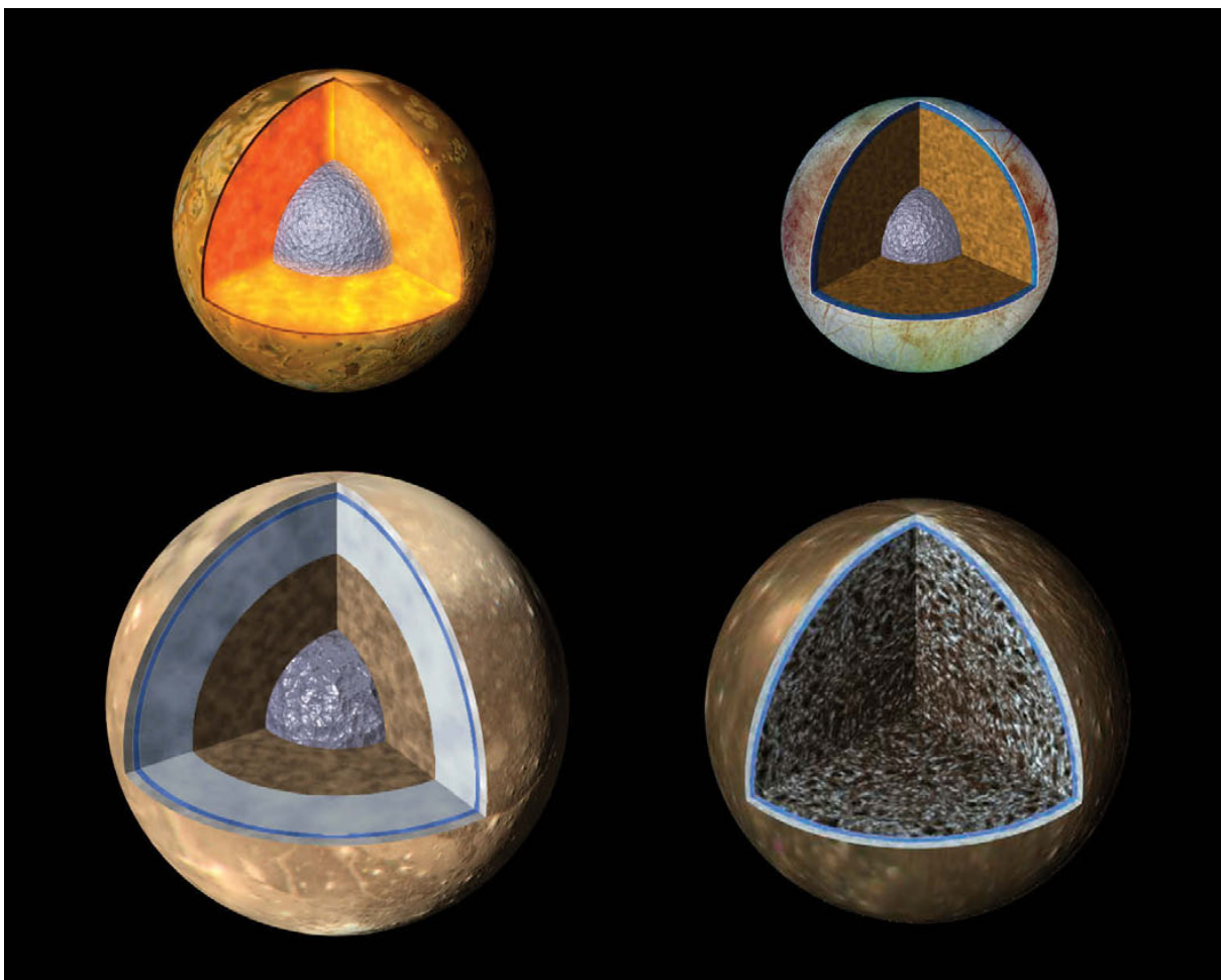
FIGURE 8.2 Schematic of the highly diverse interiors of the Galilean satellites, inferred from Galileo data. Io ( upper left ), Europa ( upper right ), and Ganymede ( lower left ) have metallic cores surrounded by silicate mantles that, in the case of Europa and Ganymede, are overlain by water ice and subsurface oceans (blue). Europa's ocean, unlike Ganymede's, is in contact with the underlying silicate mantle. Callisto ( lower right ) also hosts an ocean but is only partially differentiated, and its interior consists primarily of mixed silicates and ice. Ganymede's diameter is 5,262 km. SOURCE: NASA/JPL.
