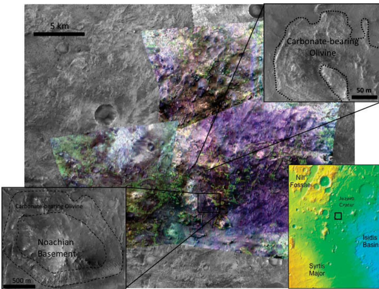
FIGURE 6.3 Diverse mineralogy, observed with Compact Reconnaissance Imaging Spectrometer for Mars (CRISM) data, formed by water-related processes and indicative of potentially habitable environments. SOURCE: B.L. Ehlmann and J.F. Mustard, Stratigraphy of the Nili Fossae and the Jezero Crater Watershed: A Reference Section for the Martian Clay Cycle, presentation at the First International Conference on Mars Sedimentology and Stratigraphy, April 19-21, 2010, El Paso, Texas, #6064, Lunar and Planetary Science Conference 2010. Lunar and Planetary Institute.
