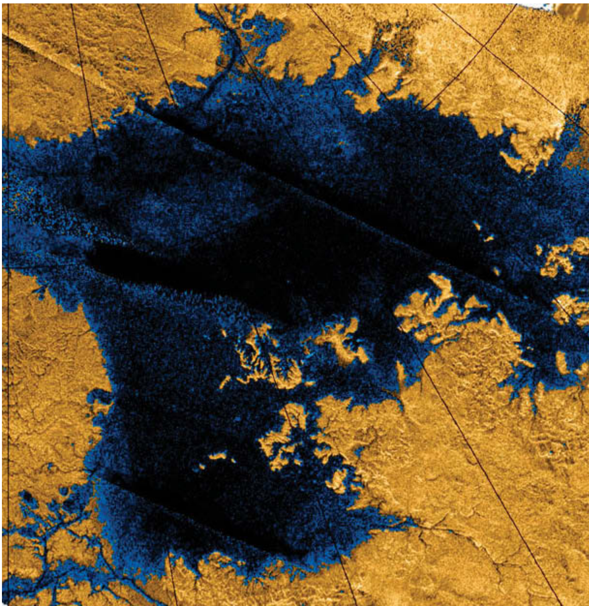
FIGURE 8.3 False-color Cassini radar image of a methane sea near Titan’s north pole, fed by dendritic drainage channels. The image is 360 km from top to bottom. SOURCE: NASA/JPL/USGS.
