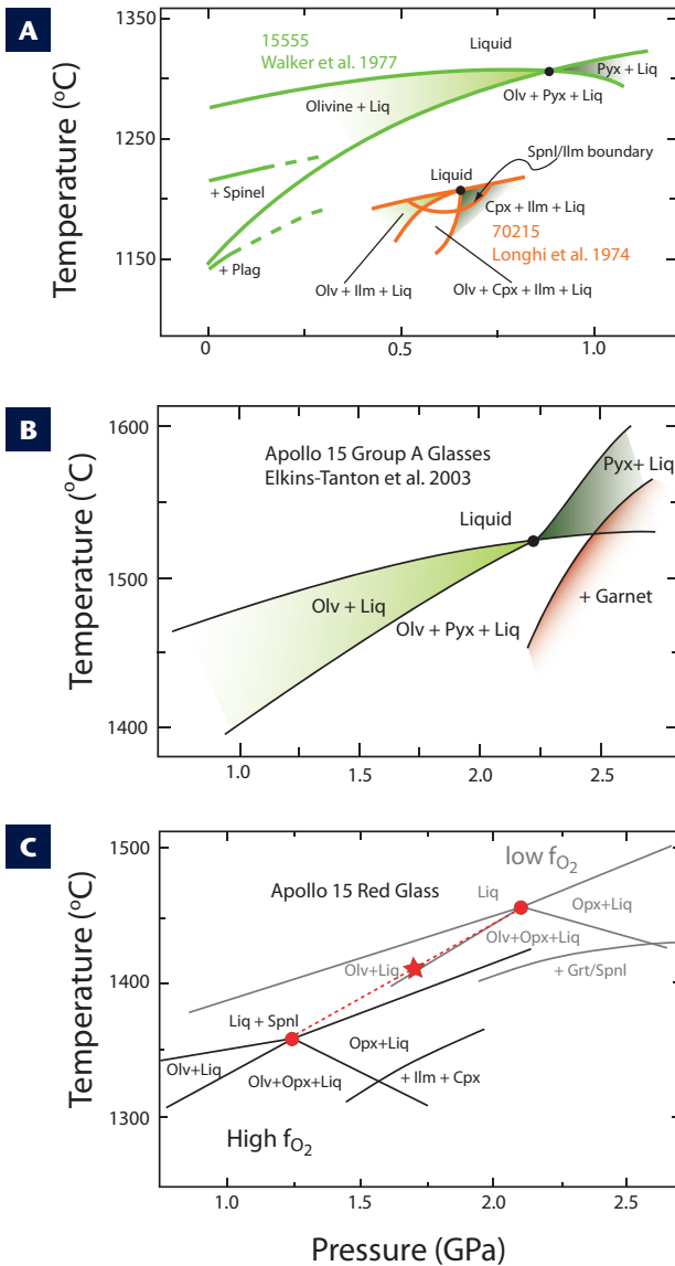
FIGURE 3 Phase diagrams for lunar mare basalts and ultramafic glasses showing the melting and crystallization behavior as a function of pressure and temperature. (A) Phase relations for Apollo 15 low-Ti mare basalt 15555 and Apollo 17 high-Ti basalt 70215 illustrate the low-pressure (lower than the ultramafic glasses) multiple-saturation, characteristic of the mare basalts and indicative of possible shallow reequilibration. (B) Apollo 15 low-Ti ultramafic glass ( \text{TiO}_2 = 0.25 wt%) shows multiple saturation at high pressure, consistent with melting of cumulates at the base of the magma-ocean cumulate pile. (C) Apollo 15 red glass ( \text{TiO}_2 = 13.8 wt%) shows the effects of oxidation state on its multiple-saturation pressures. At the inferred low oxidation state of the lunar interior, the high pressure of multiple saturation is inconsistent with melting of \text{TiO}_2 -rich cumulates that are at shallow depths in the cumulate pile.
