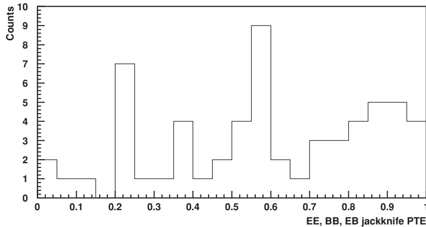
Figure 8. Probabilities to exceed the \chi^2 values from EE , BB , and EB jackknife tests are consistent with a uniform distribution between zero and one.
